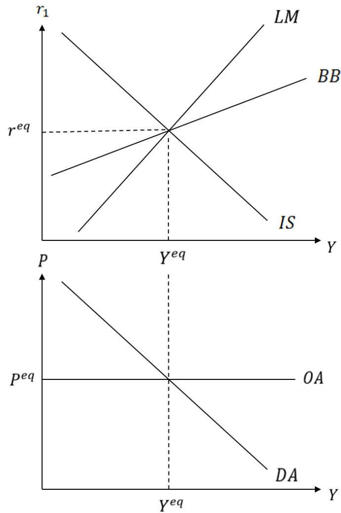
Figure 7 IS-LM-BB, aggregate supply and demand
