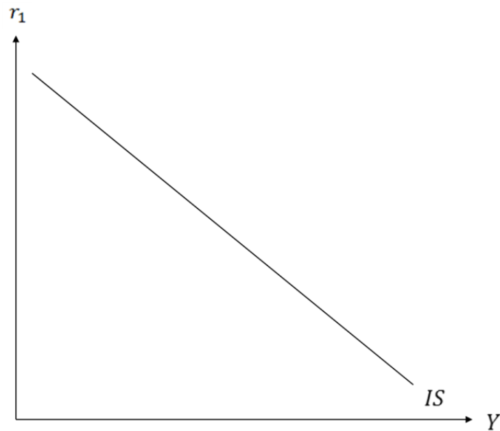
Figure 1 The IS curve
