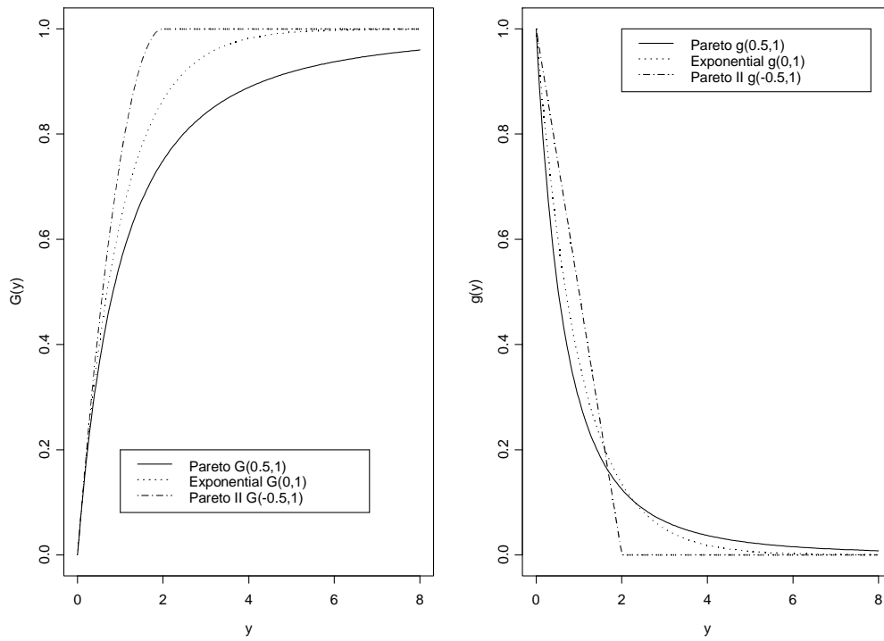
Figure 13. Generalized Pareto CDFs and pdfs for Pareto
