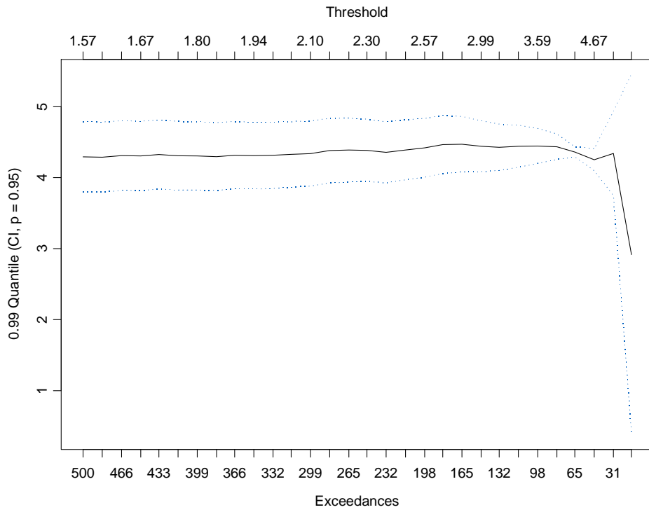
Figure 21. Estimation of the VaR_{0.99} as a function of the Threshold
